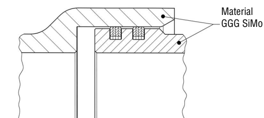
Installation situation
