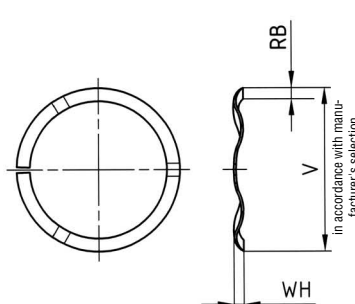
Wave spring FK9
