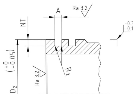
Ring carrier
