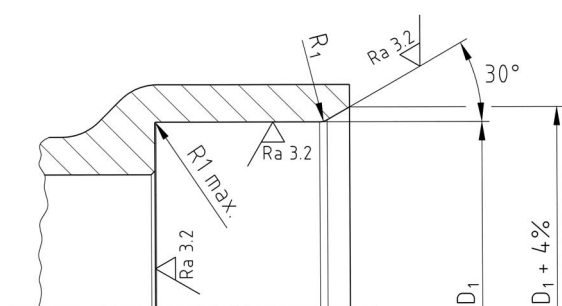
Bore/housing
